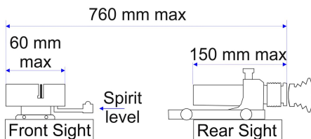
Figure F7: Sighting Equipment Limits
