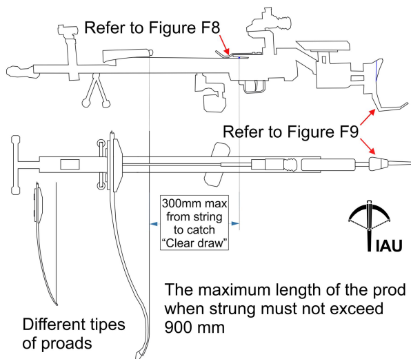
Figure F6: Target Crossbow Limits
