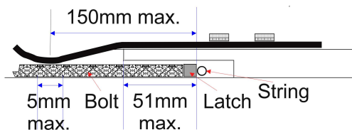
Figure F8: Bolt retainer and string guide limits
