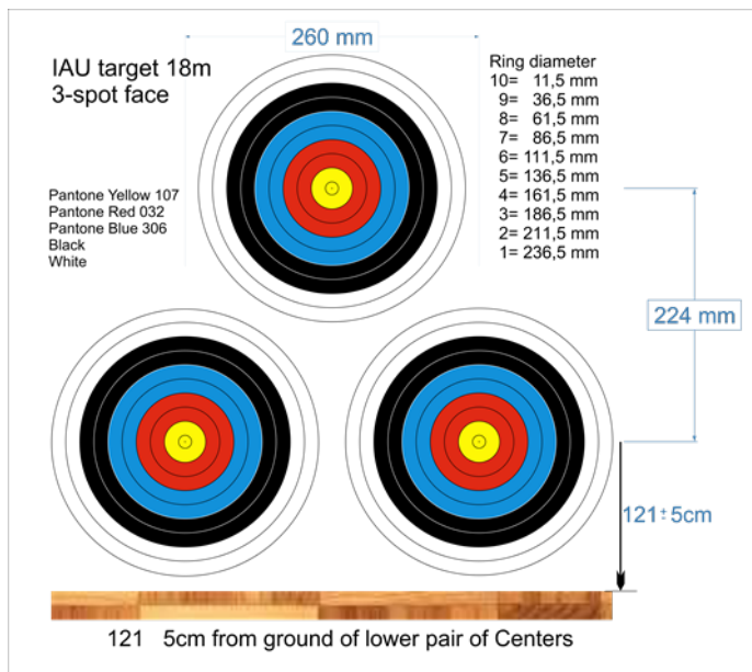
Figure F2: Field Layout (Refer to Art. 315): Indoor 18 m: 23,65 cm full ring 3-spot Target Face
