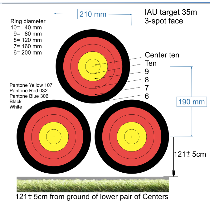
Figure F5: 40 cm 3-Spot Target Faces
