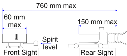
Figure F6: Target Crossbow Limits
